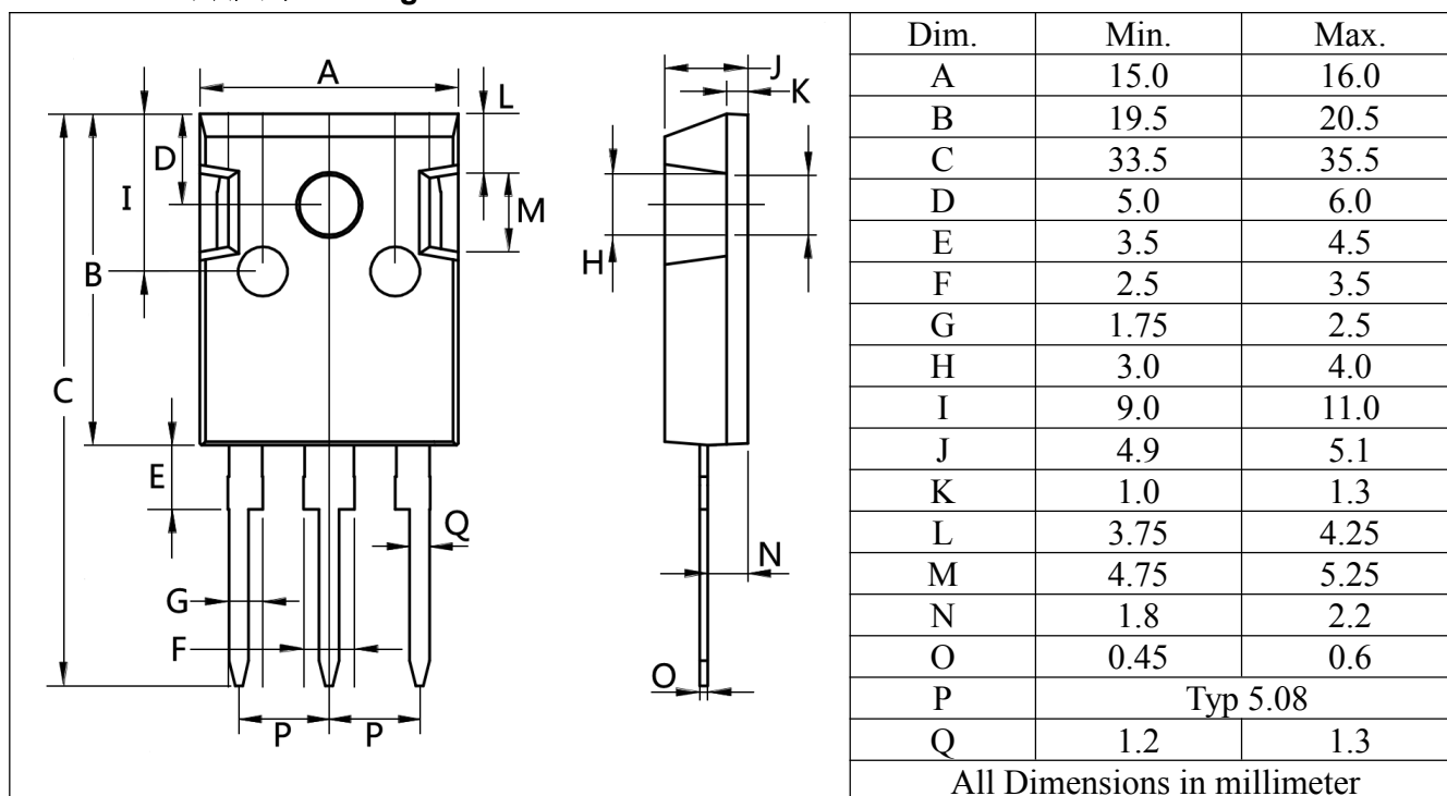
TO-247S 封装尺寸 Package size
